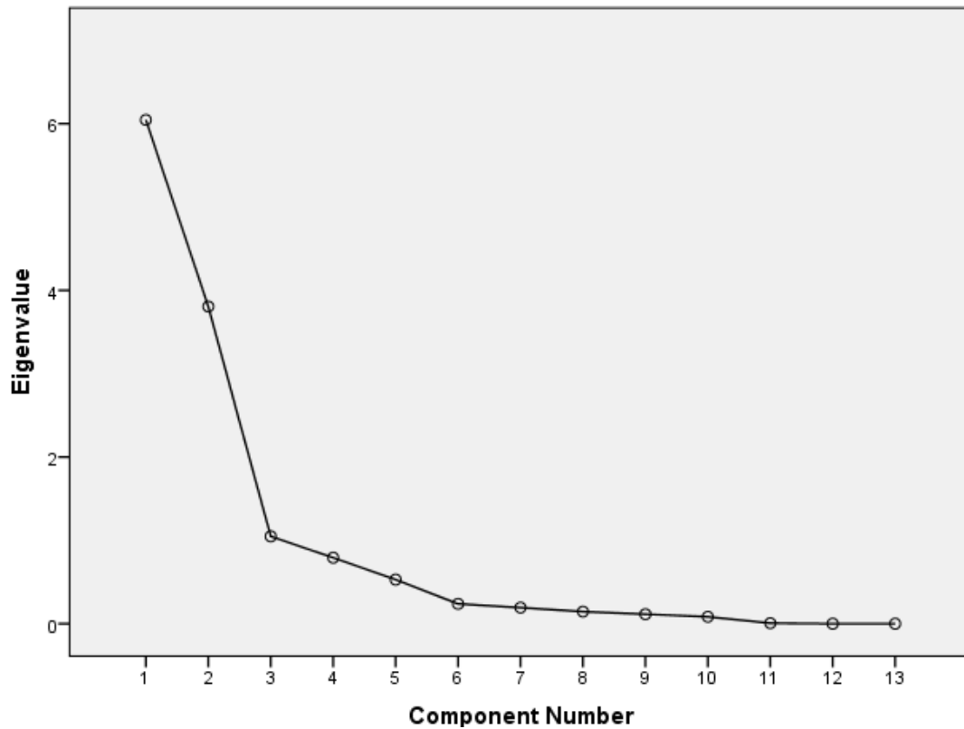
Figure 3: Scree plot
