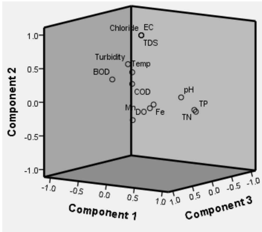
Figure 2: Component plot in rotated space
