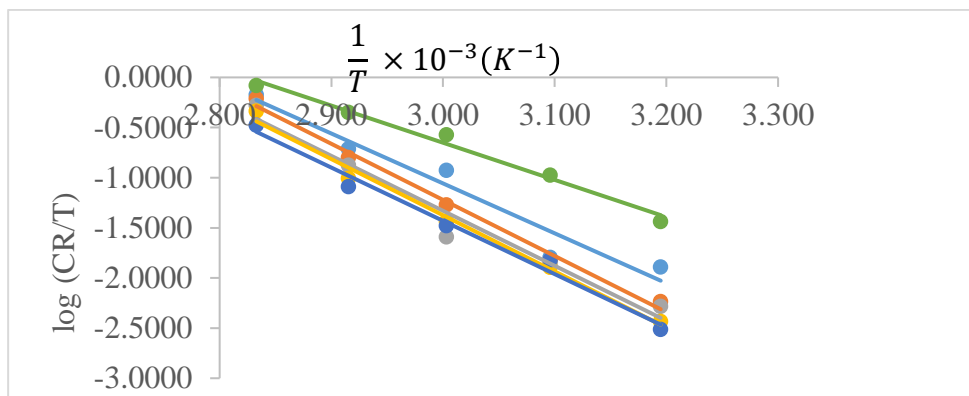
Figure 2: The transition state plot for the corrosion inhibition of stainless steel
