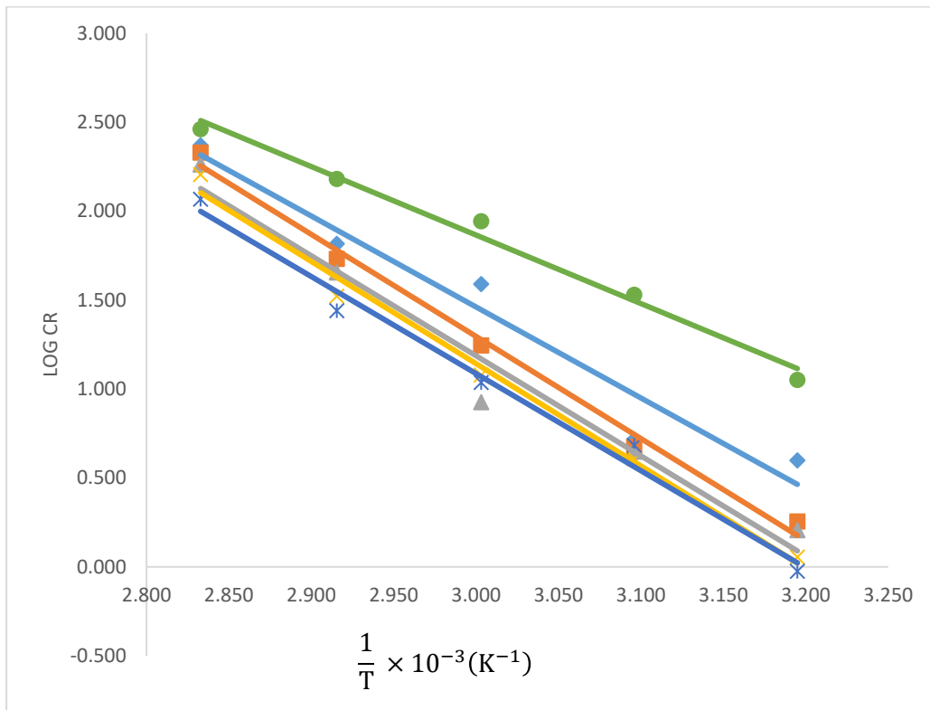
Figure 1: Plot of Arrhenius for the corrosion inhibition of stainless steel.
